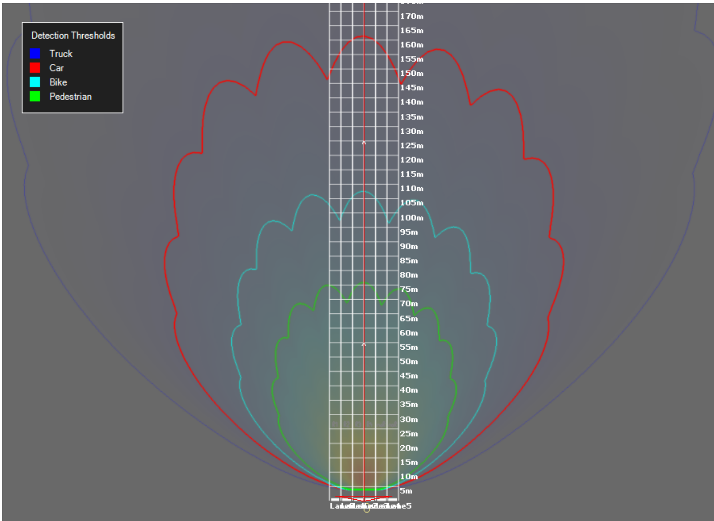
Figure 4: Beam Pattern Type 42, Range values given for 12.7dBm EIRP
