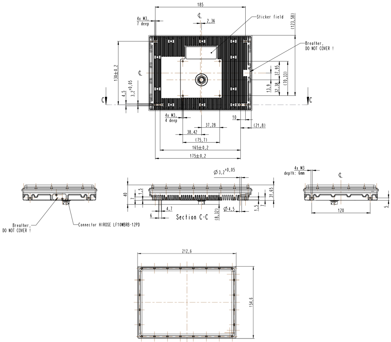
Figure 8: Sensor Dimensions.
